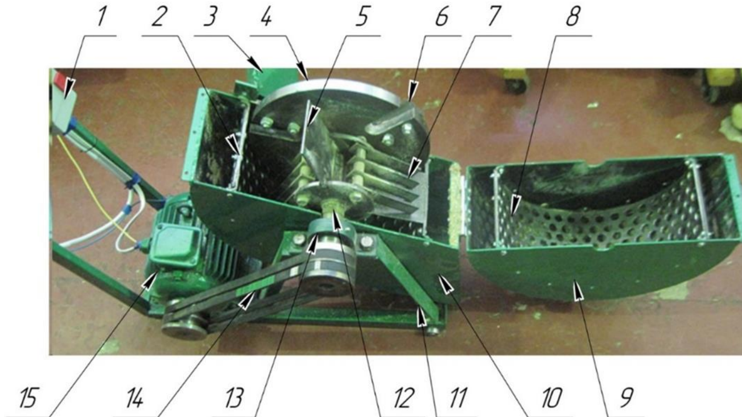
General view of the developed chopper of tree branches
