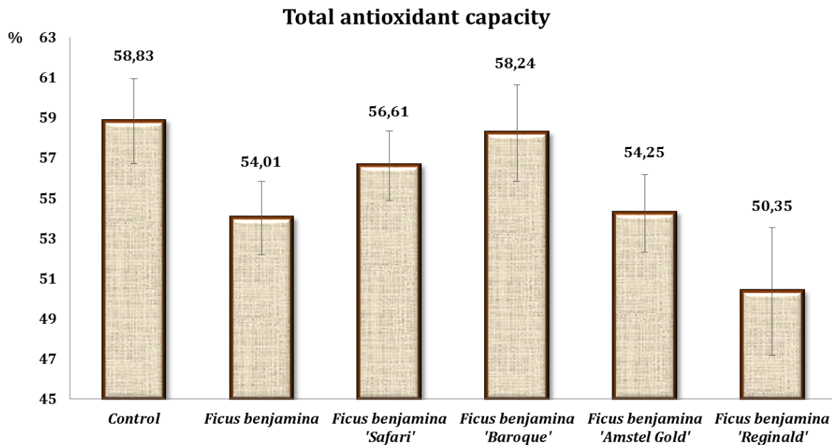
Fig. 1. The total antioxidant capacity (TAC) in the equine erythrocyte suspensions after in vitro incubation with extracts derived from leaves of Ficus benjamina and its cultivars ( M \pm m , n = 18 ).
