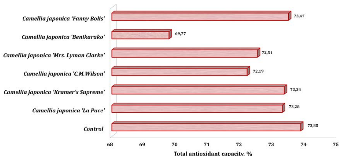
Fig. 1. The total antioxidant capacity (TAC) values in the equine erythrocyte suspensions after in vitro incubation with leaf extracts derived from Camellia japonica cultivars ( M \pm m , n = 18 ).
