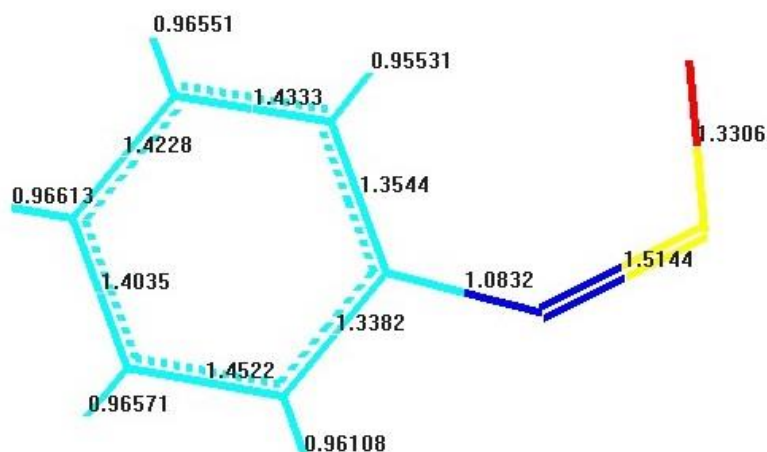
Fig. 3. Bond orders in the N-sulphinylamine molecule in the ground singlet state
