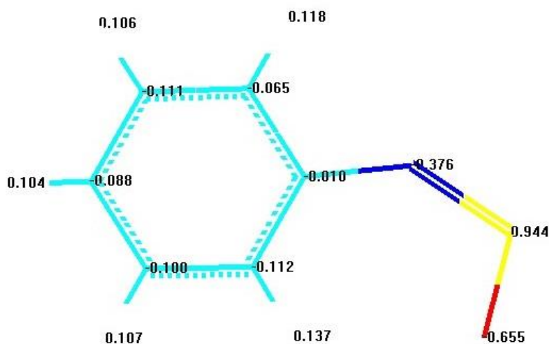
Fig. 2. Atomic charges in the N-sulphinylaniline molecule in the ground singlet state (charge N = -0.376 )
